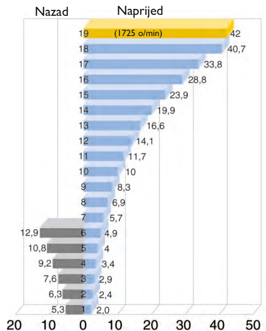
Power Command™ – Full Powershift*
