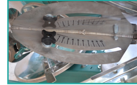
Skala za podešavanje preciznog rasipanja Setting gauge corresponding to the spreading charts for highly accurate fertilization
