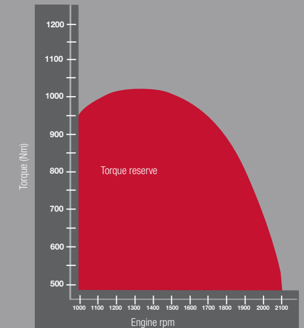
This curve clearly shows how maximum torque is maintained between 1200 and 1500 rpm, with steep torque rise as engine rpm falls between 2100 and 1500 rpm for greater torque ability and constant PTO speed.
