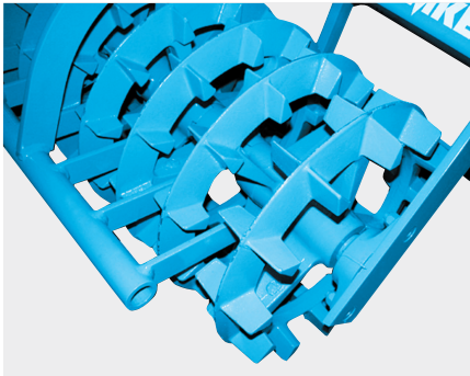
Crosskill Roller
