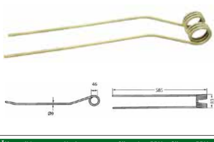
Opruga sakupljača Pottinger: TOP 42, 420, 460, 770, Eurotop 421, 461, 601, 691, 770, 771
