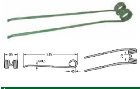
Opruga sakupljača Stoll: 281, 282, 311, 331, 371, R281, R282, R311, R331, R371
