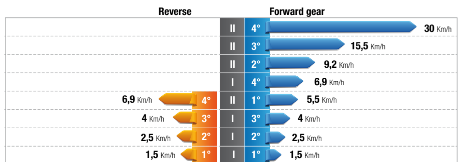
GRAPH OF SPEEDS IN KM/H WITH 210/95R16 TYRES OF THE AR AND RS VERSION TRACTORS.
