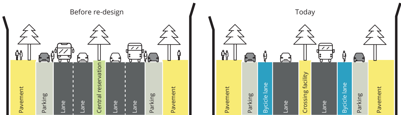
FIGURE 11.6 Redesign of roadways in Berlin to reduce traffic noise: before and after
