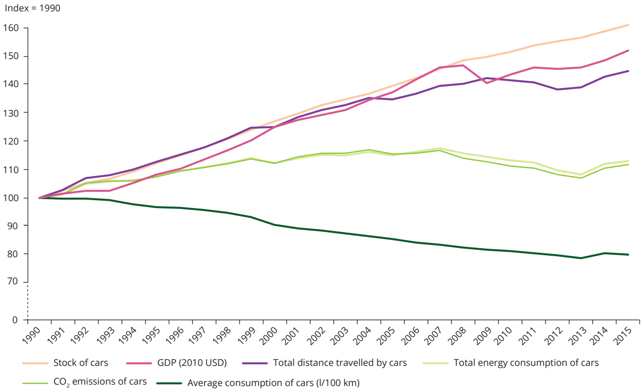
FIGURE 16.5 Fuel efficiency and fuel consumption in private cars, 1990-2015
